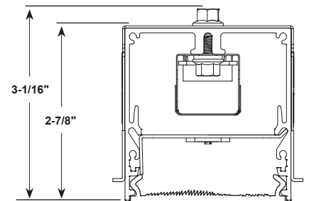
ASYMMETRIC DIFFUSER
