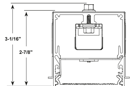
BATWING DIFFUSER
